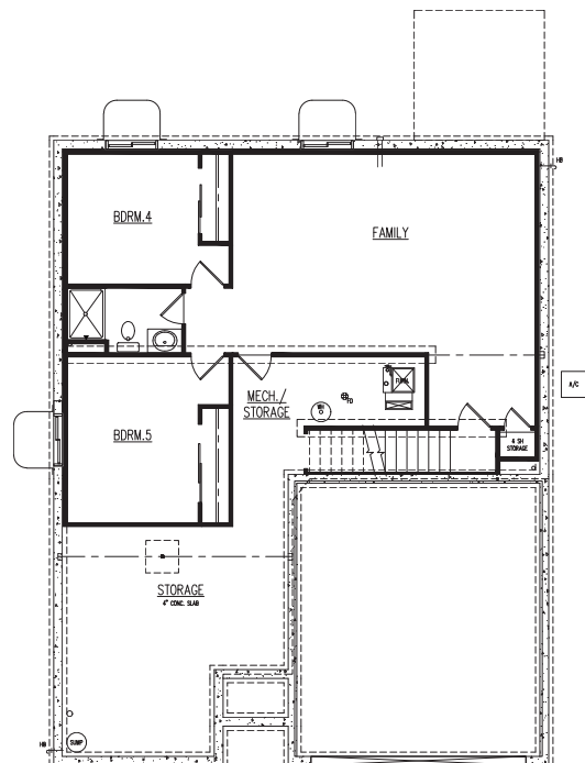
LOWER LEVEL (proposed)
