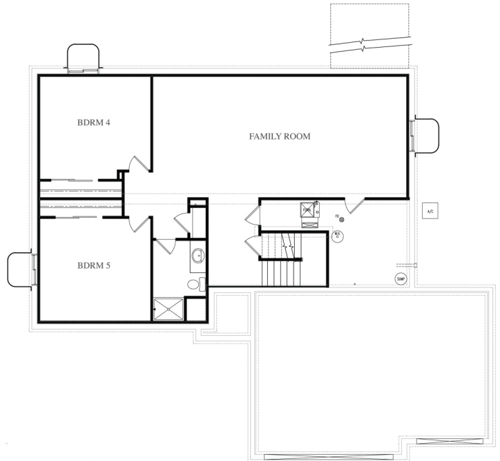
BASEMENT {proposed}
